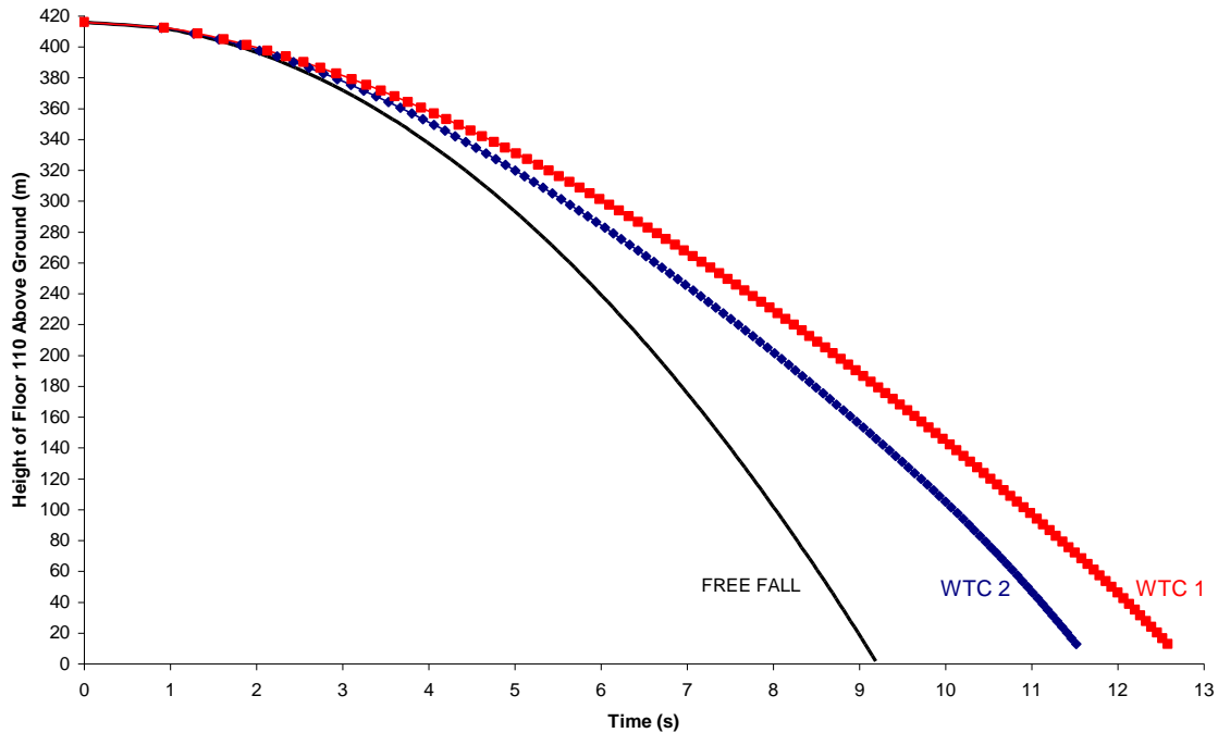
Figure 1: WTC TOWERS 1 and 2 COLLAPSE PROFILES
